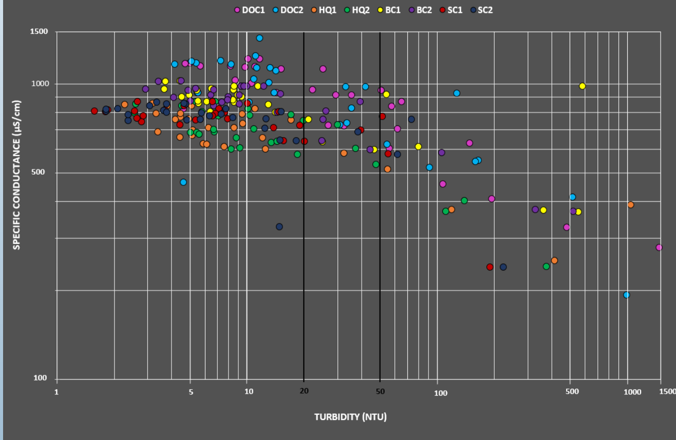
Above: Creek site turbidity and specific conductance, from December 2019-September 2020. Turbidity limits are presented in black.
